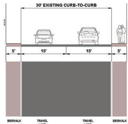
Figure 80. Saratoga Avenue Existing Typical Section From Bay Road To Newbridge Street (Facing North)
