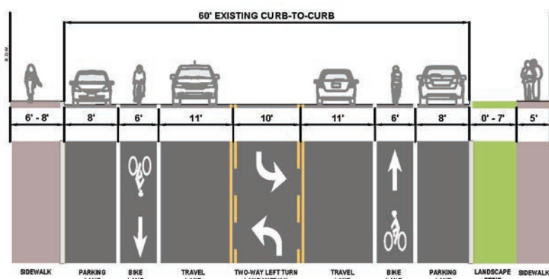
Figure 65. Industrial Road Existing Typical Section E (Facing North)
