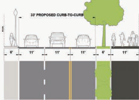
TYPICAL SECTION A
