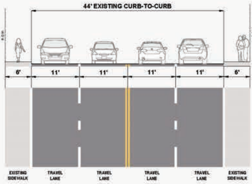
SAN BRUNO AVENUE - EXISTING TYPICAL SECTION SAN MATEO AVENUE TO 7TH AVENUE
