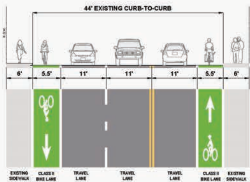
SAN BRUNO AVENUE - PROPOSED TYPICAL SECTION SAN MATEO AVENUE TO 7TH AVENUE
