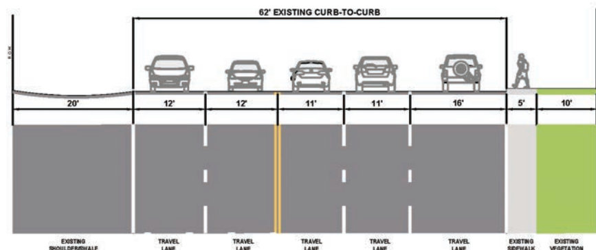
Figure 48. San Bruno Ave Existing Typical Section From US 101 To McDonnell Road (Facing East)
