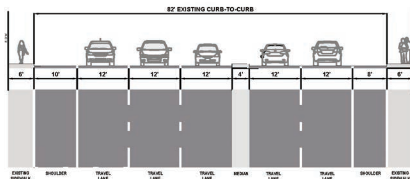
Figure 47. San Bruno Ave Existing Typical Section Over US 101 Overcrossing (Facing East)
