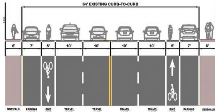
Figure 61. Industrial Road Existing Typical Section A (Facing North)
