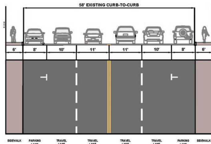
Figure 71. Bay Road Existing Typical Section From Woodside Road To Second Avenue
