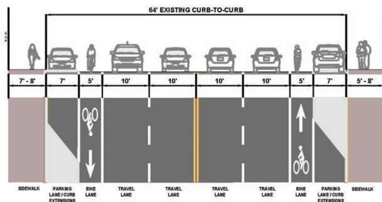
Figure 64. Industrial Road Existing Typical Section D (Facing North)
