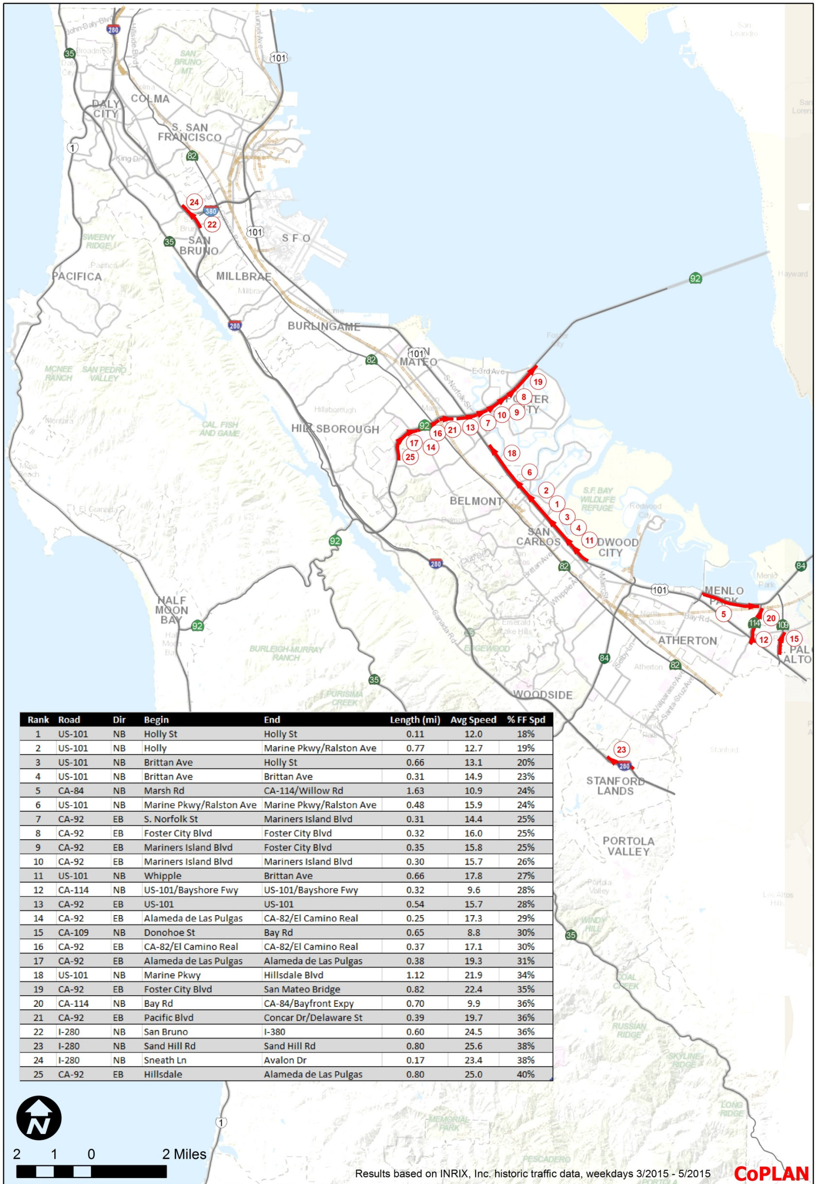
Worst 25 Segments based on Travel Speed (Percent of Free Flow) : Evening Peak Hour (5-6 PM)
